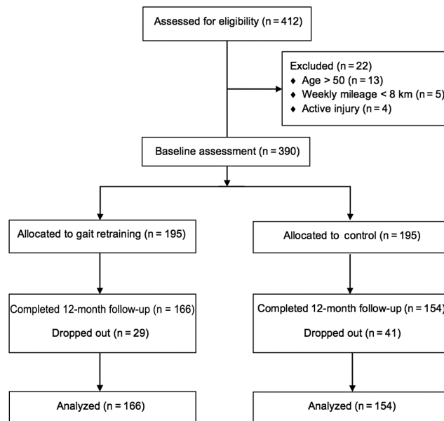
Figure 3. Consort diagram.
