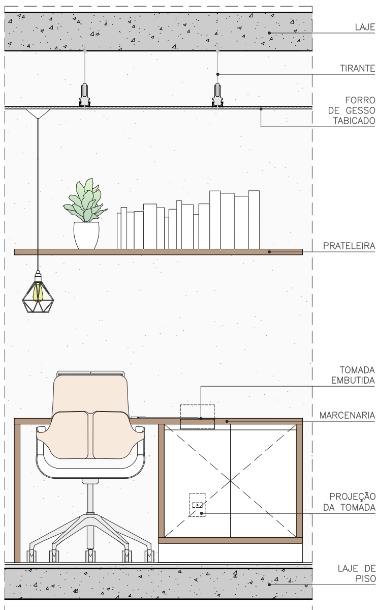
VISTA FRONTAL
