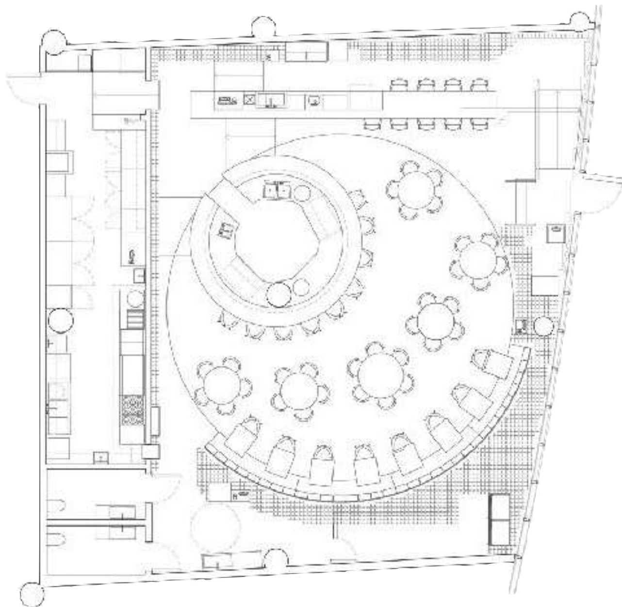
FLOOR PLAN
